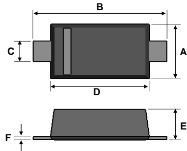
SOD-123F
